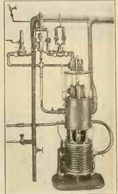
FIG. 7.—SECTIONAL TANDEM 9 1/2 INCH HEAD AND PUMP.
